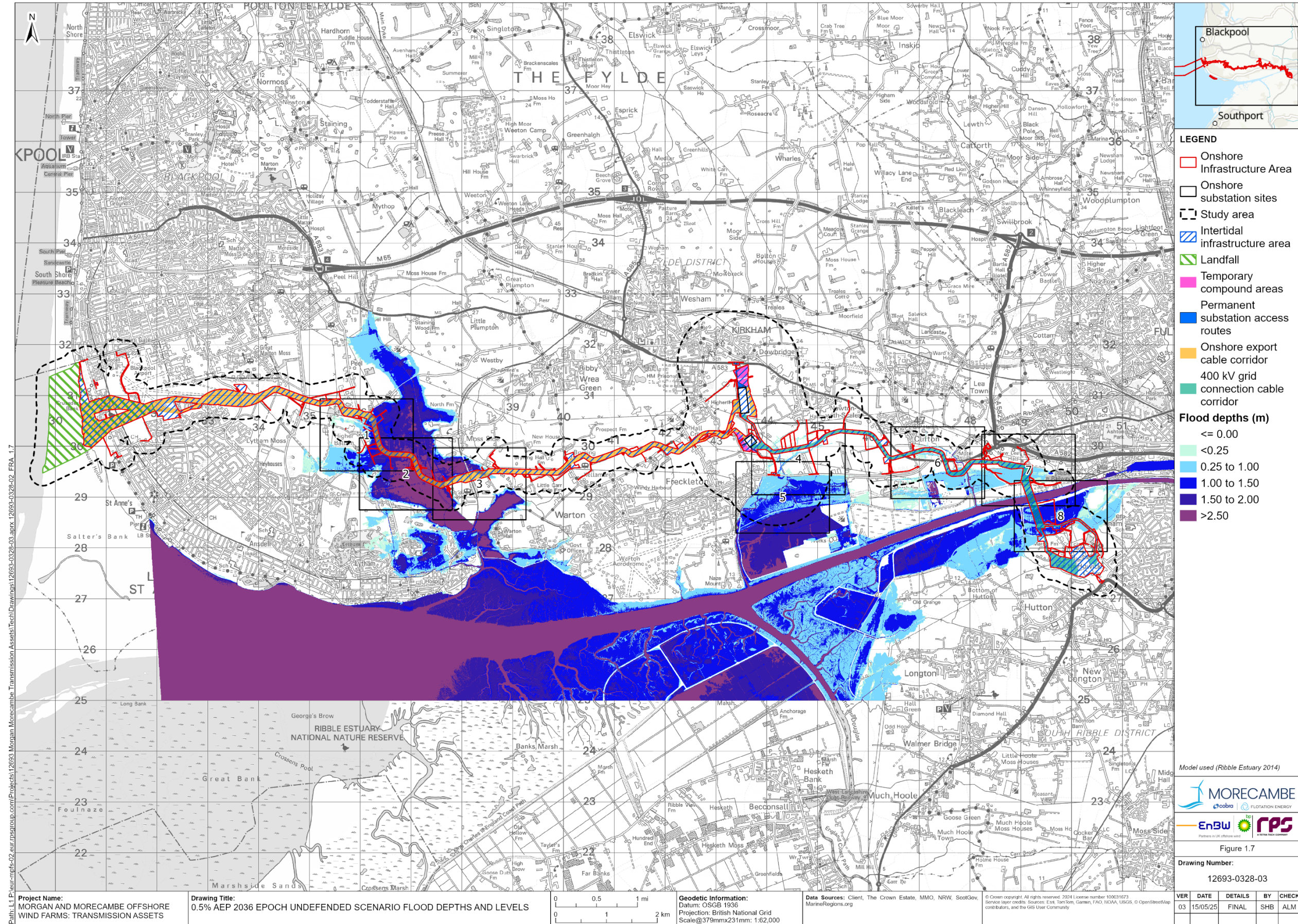
Figure 1.7: 0.5% AEP 2032-2036 epoch undefended scenario flood depths and levels
